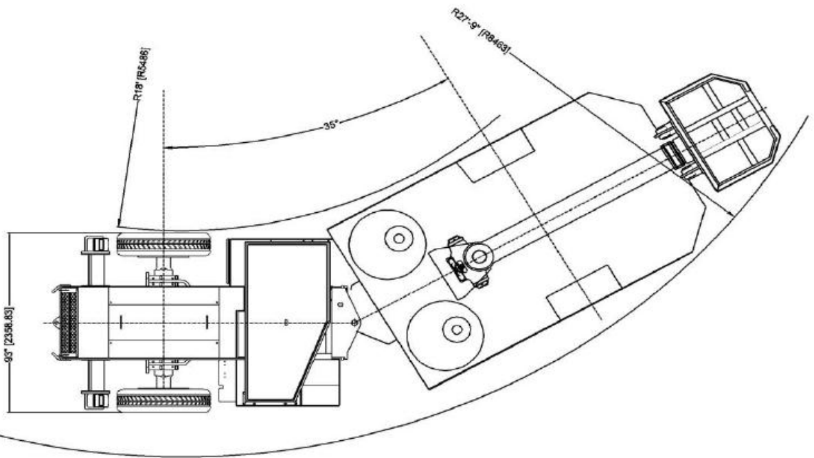
TURNING RADIUS
